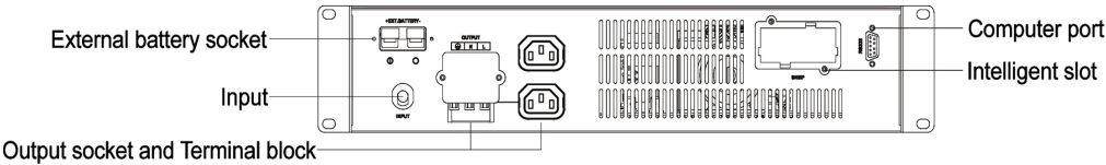
PT-RT1-3K/1-3KL Rack Mount Rear Panel
