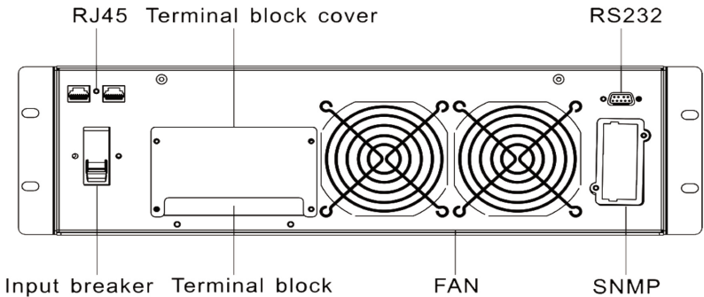
BACK VIEW OF 10KL
